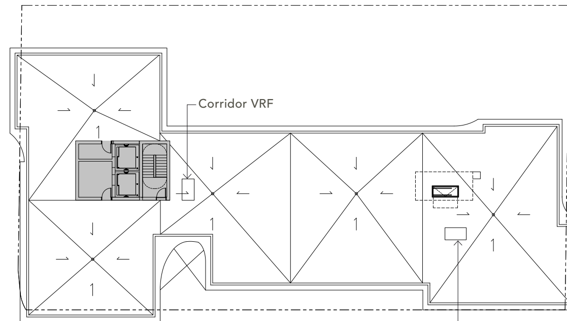
Roof Plan
