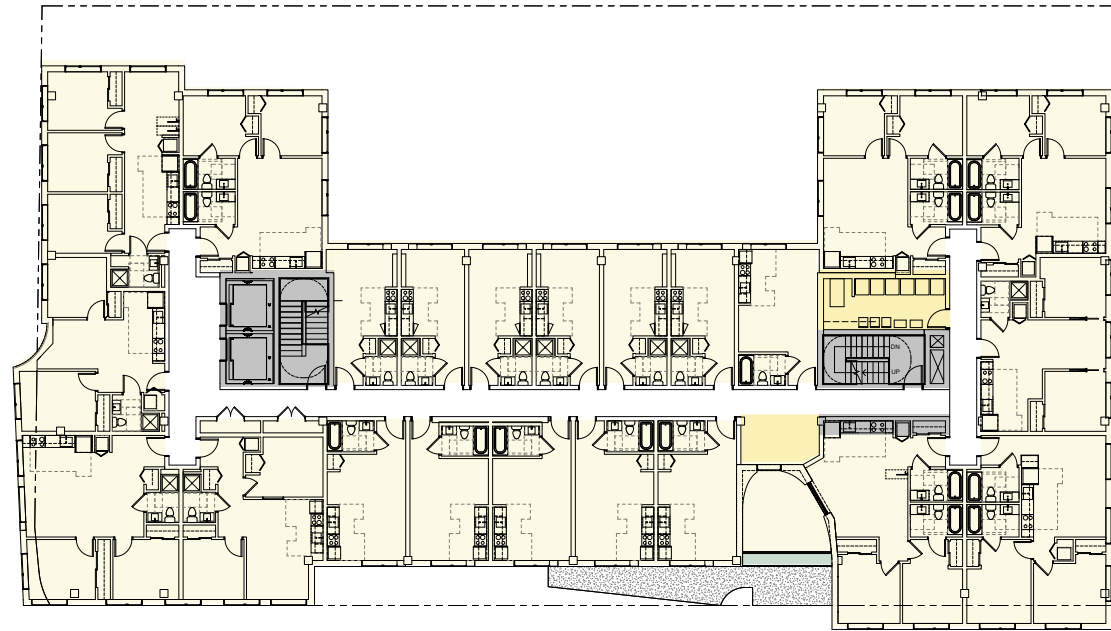
Second Floor
