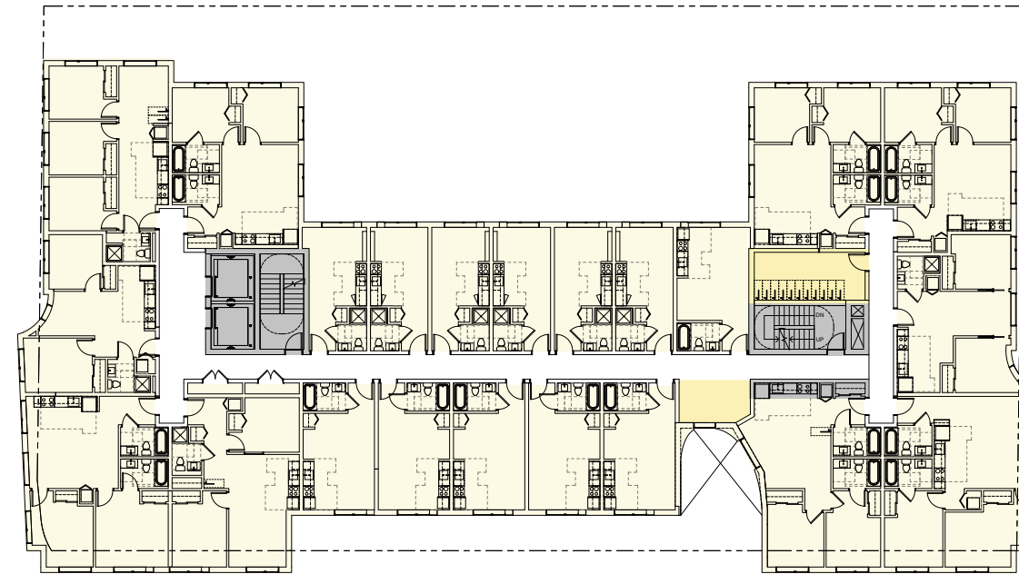
Fourth Floor
