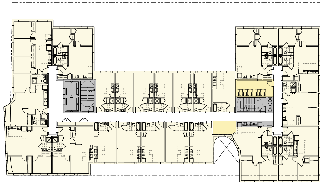
Third Floor
